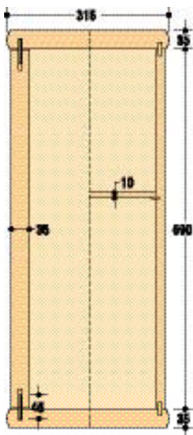
SPLIT SECTION 1:10
